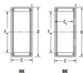
Boundary dimensions
