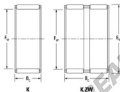
ISO 300 Needle roller and cage assemblies
