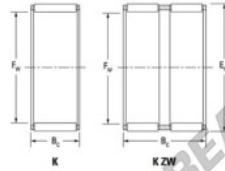
Partial inside roller and cage assemblies
